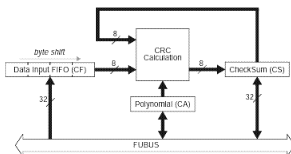
Figure 40-9. CRC Structure
