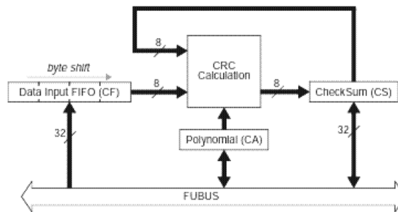
Figure 40-9. CRC Structure
